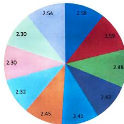
3-Scale Index
