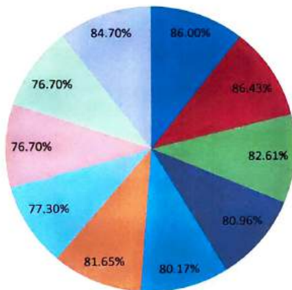
Percentage
